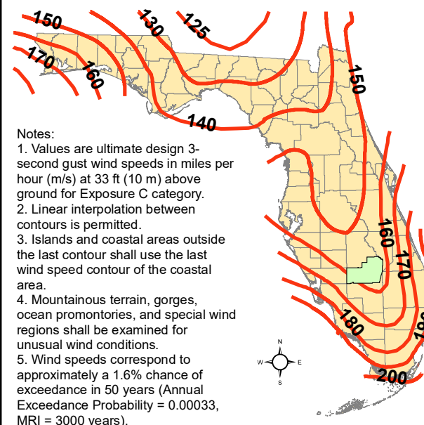
Figure 1609.3(3) Ultimate Design Wind Speeds, for Risk Category IV Buildings and Other Structures
